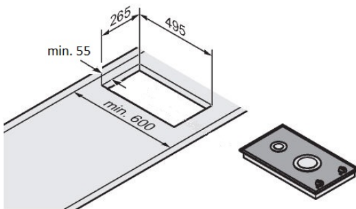
GKS 6940.0 installation dimensions
