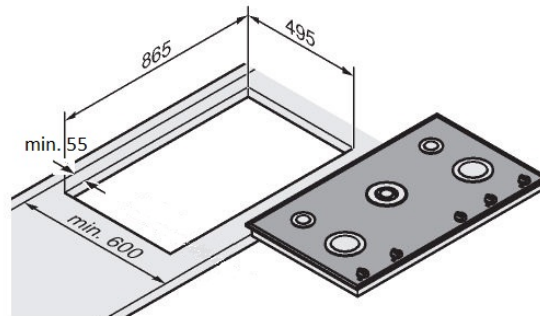
GKS 9951.0 installation dimensions
