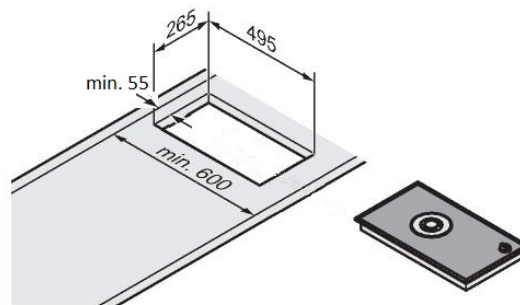
GKS 9951.0 installation dimensions
