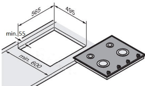
GKS 6940.0 installation dimensions
